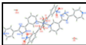
Fig. 1. A view of the molecular structure of ( I ) with the atom-numbering scheme and 30% displacement ellipsoids (arbitrary spheres for the H atoms). Atoms with the suffix A are generated by the symmetry operation ( -x + 2, -y + 1, -z + 1 ).
